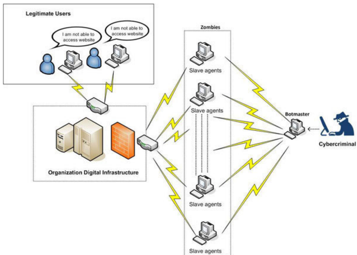
Figure 2.3: Distributed denial-of-service
