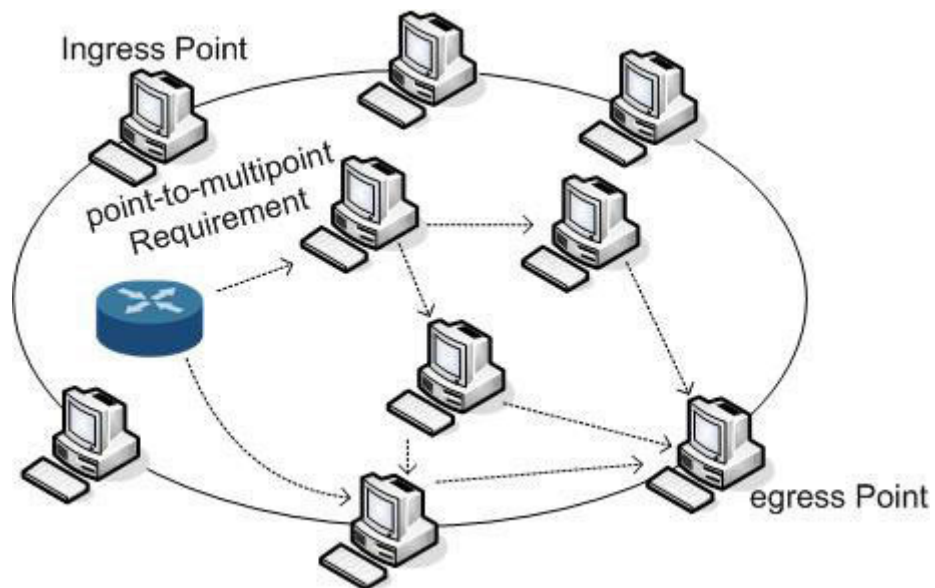
Figure 5.8: Demand matrix
