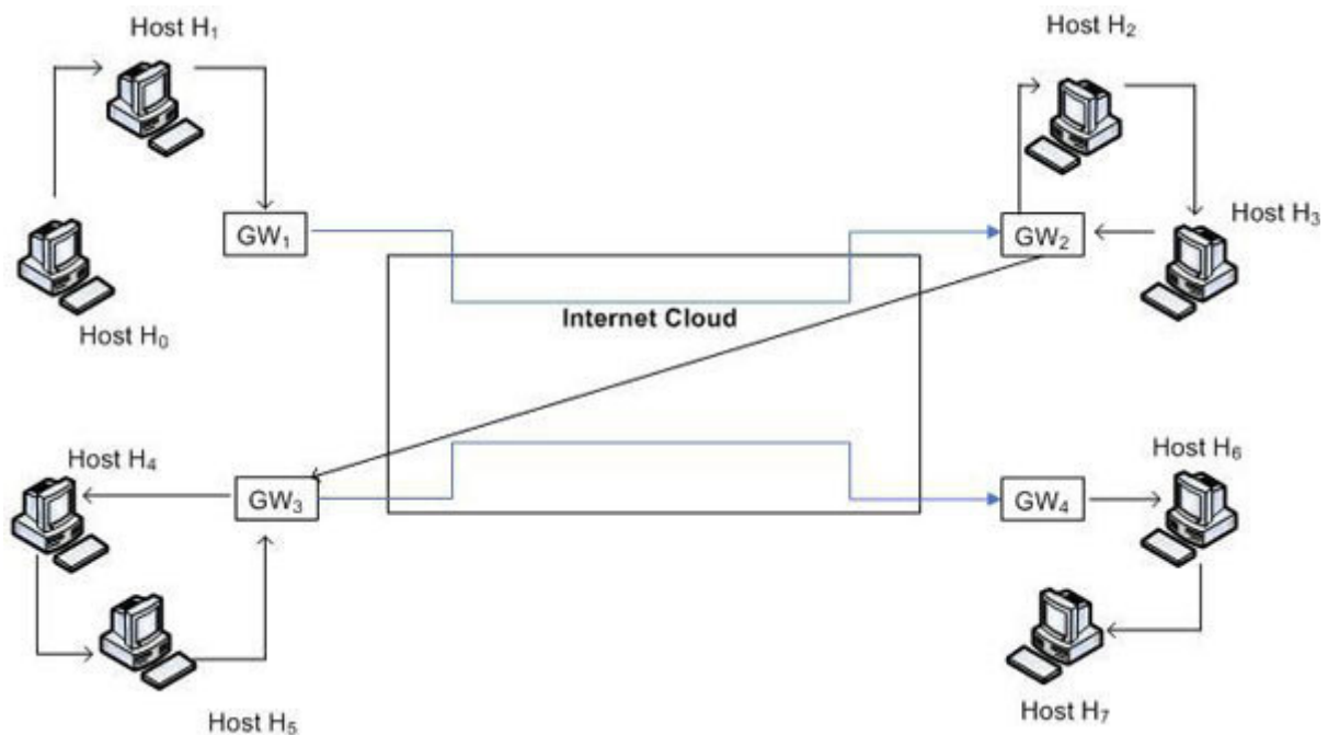
Figure 4.11: Tracing model
