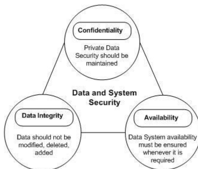
Figure 3.1: CIA triad
