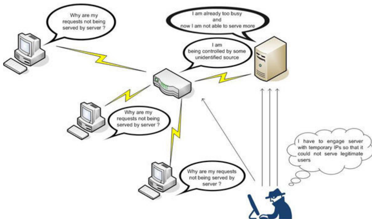
Figure 2.2: Denial-of-service attack
