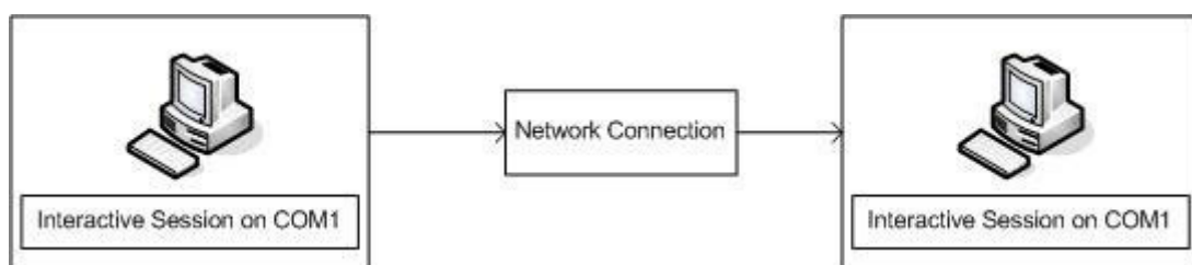
Figure 5.1: Session management
