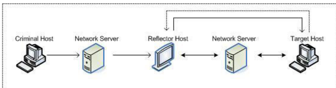
Figure 4.3: Reflector host
