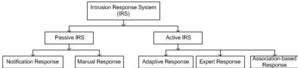
Figure 5.9: IRS classification
