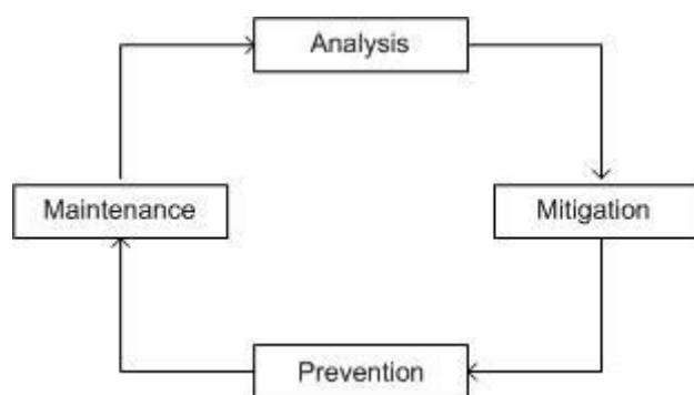
Figure 3.2: Defensive life-cycle
