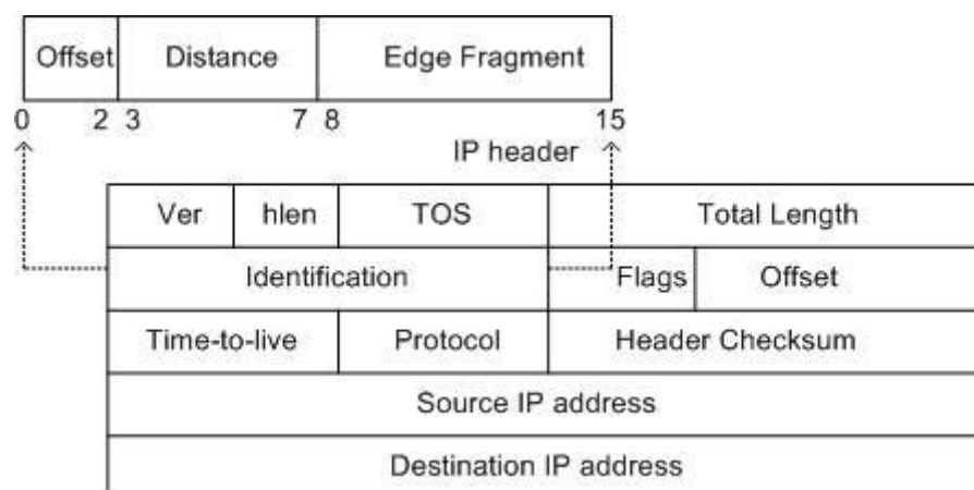
Figure 4.5: IP header
