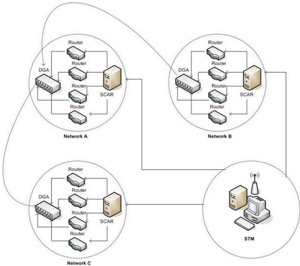
Figure 4.8: SPIE architecture
