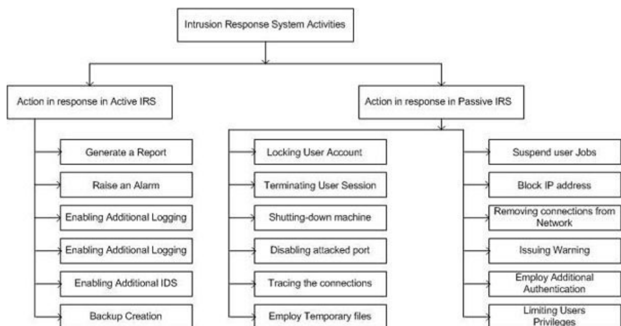
Figure 5.10: IRS actions
