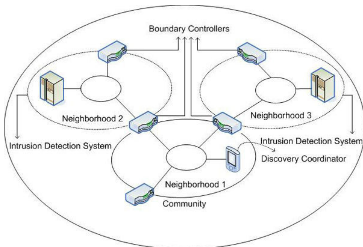
Figure 6.2: CITRAArchitecture
