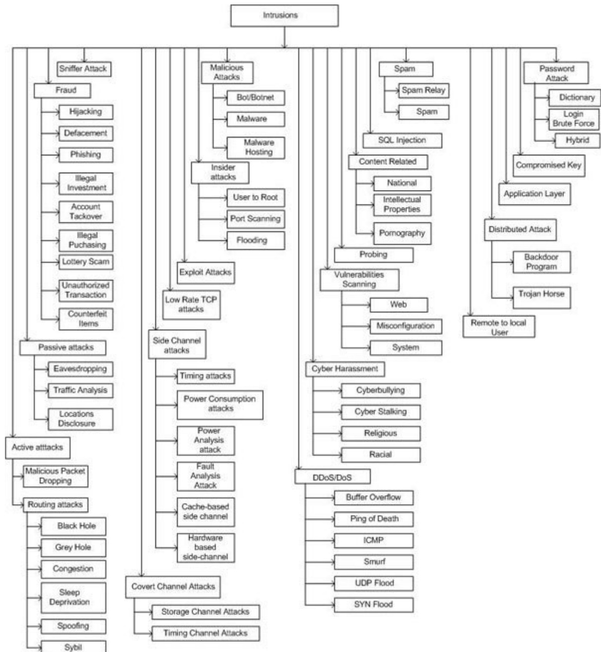
Figure 3.3: Intrusion Categories
