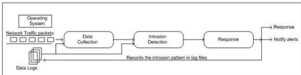
Figure 3.4: Intrusion Detection System
