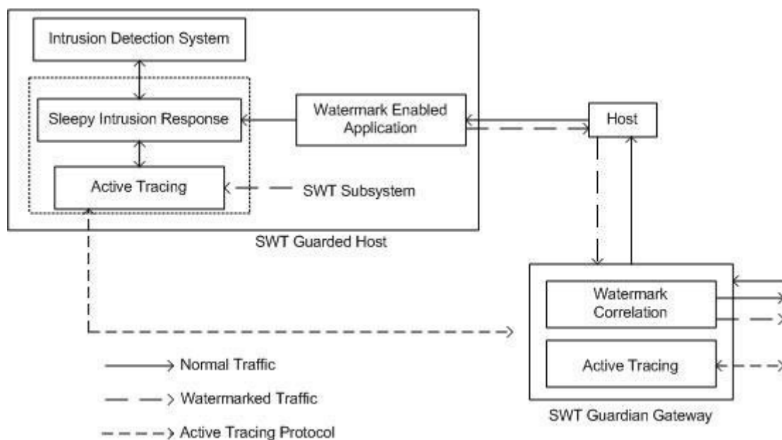
Figure 4.12: SWT architecture
